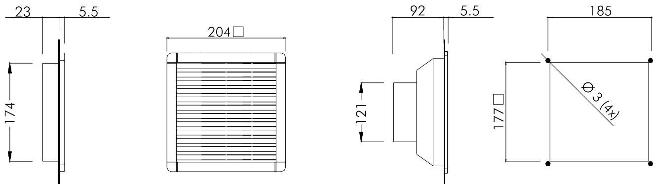
REFERENCE - FILTER FAN MVPI20
