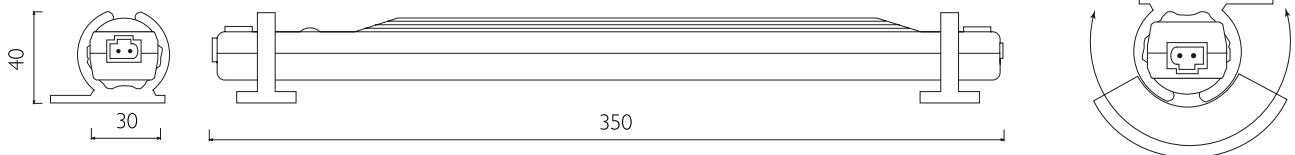
LUMINAIRE MULTIPOSITION LED 6W
